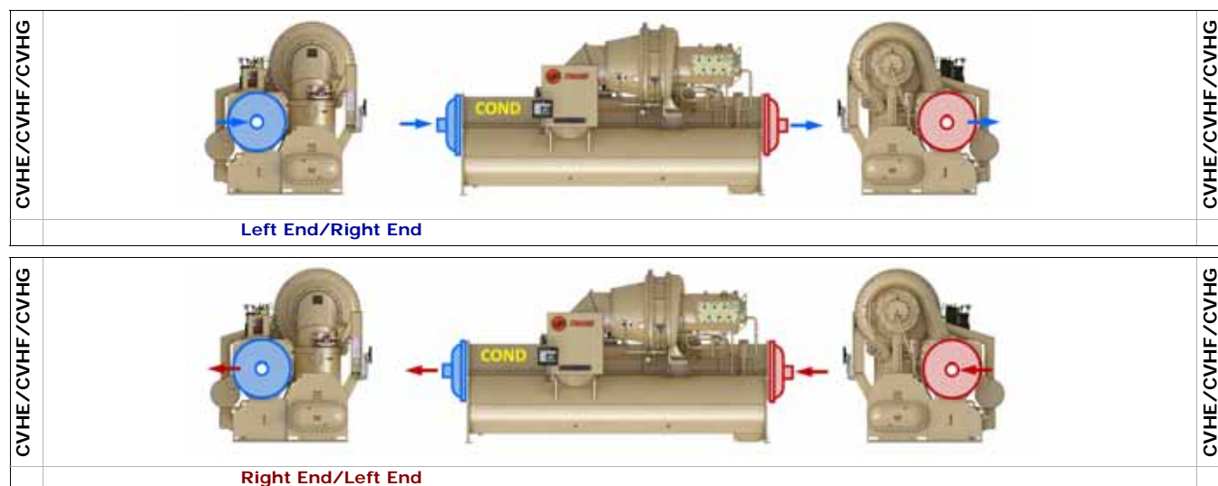
Figure 47. One-pass non-marine
