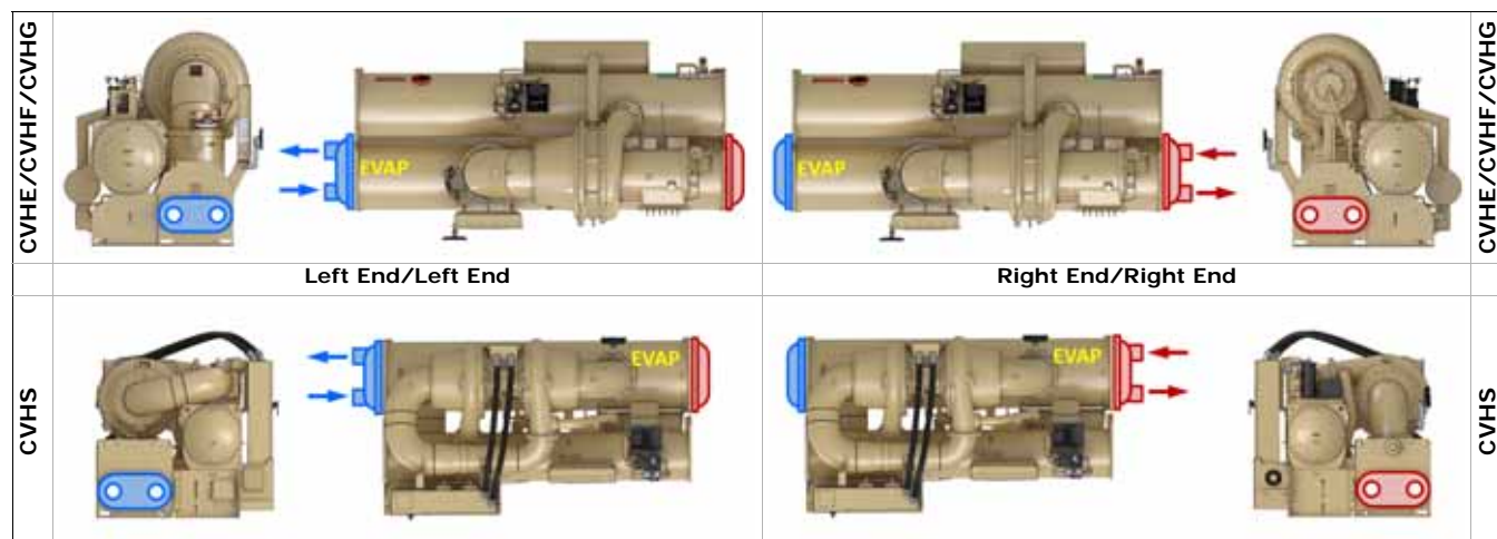
Figure 40. Two-pass non-marine
