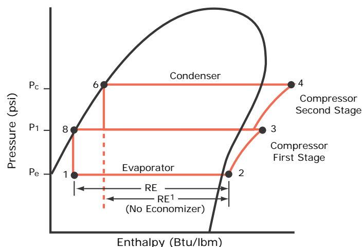
Figure 5. Two-stage CenTraVac™ chiller P-H diagram
