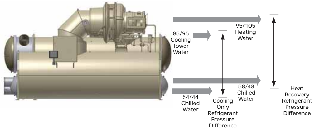
Figure 32. Chilled-water reset
