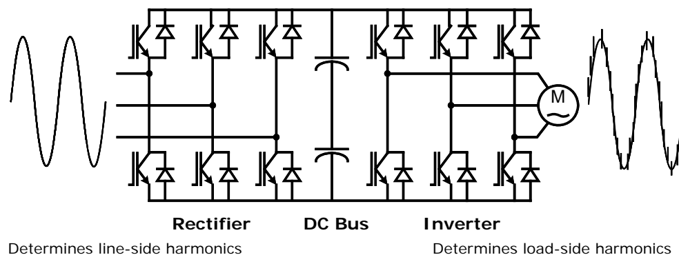
Figure 10. AFD power sections
