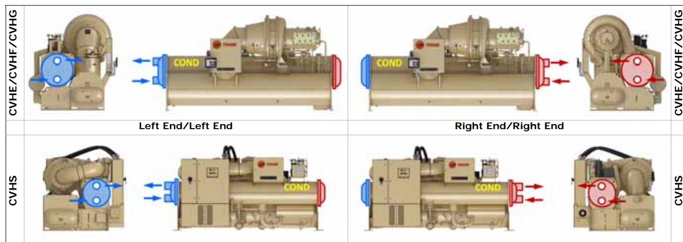
Figure 46. Two-pass non-marine
