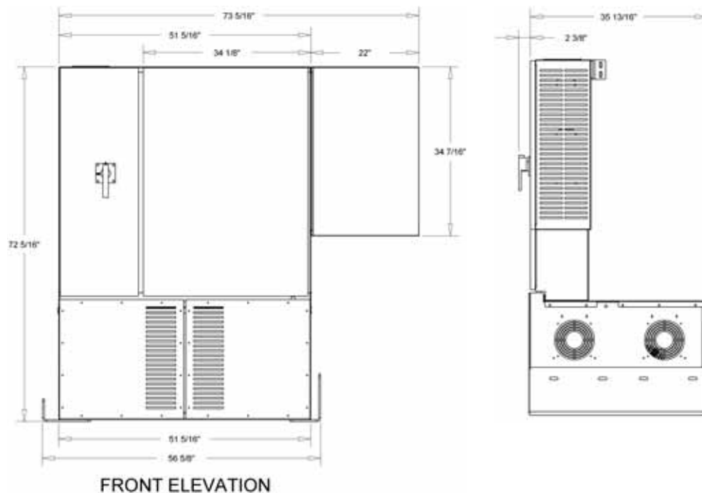
Figure 17. AFD3 dimensions—CVHS
