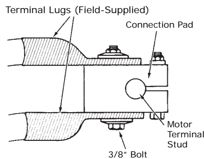
Figure 29. Electric connections
