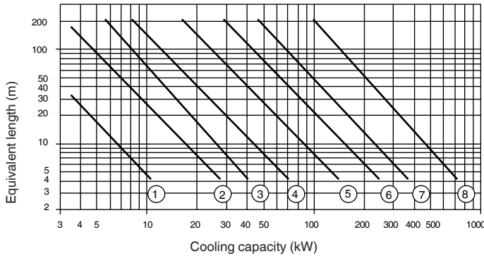
Discharge piping
