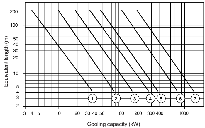
Liquid piping
